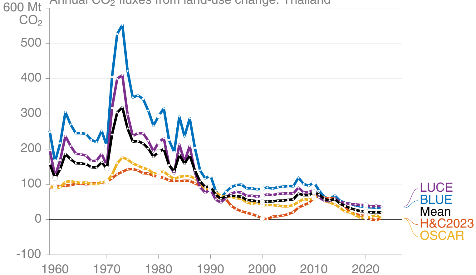
Annual CO 2 fluxes from land-use change: Thailand
