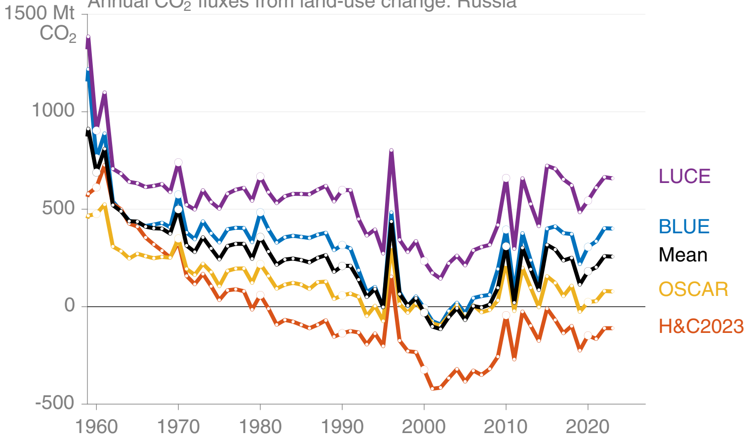
Annual CO 2 fluxes from land-use change: Russia
