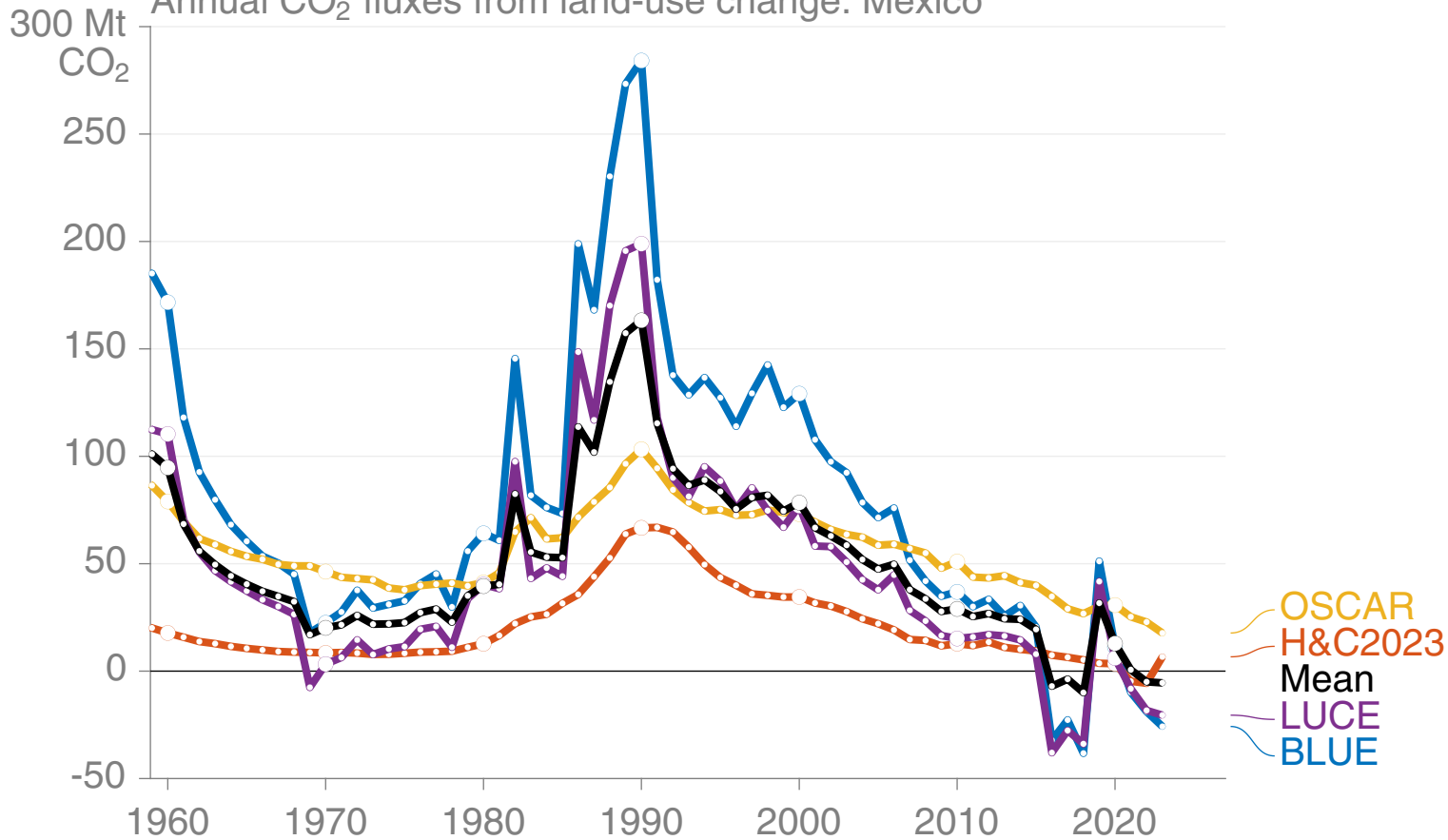
Annual CO 2 fluxes from land-use change: Mexico
