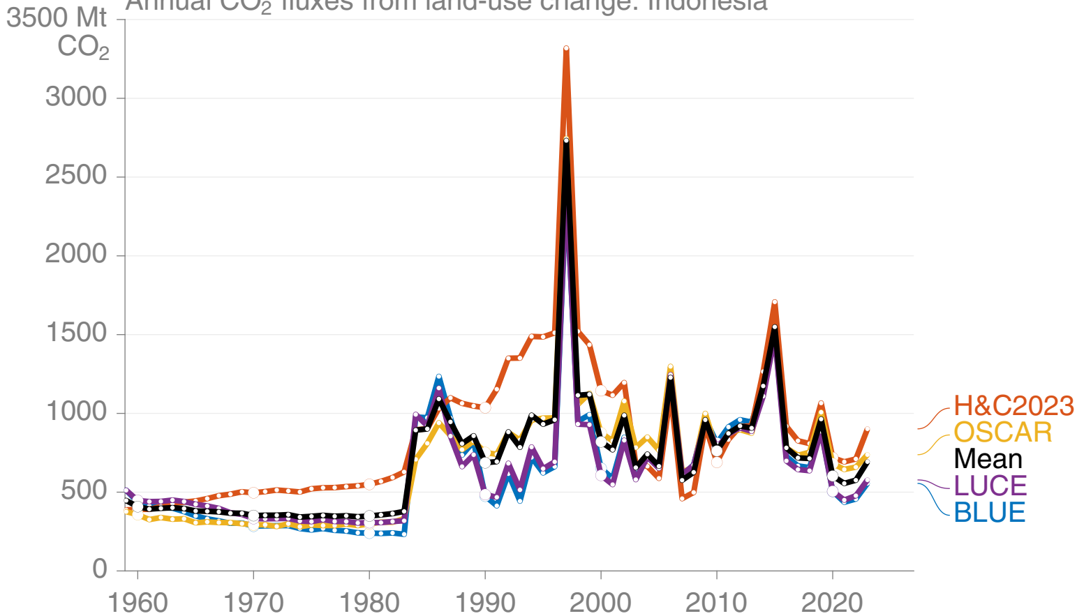
Annual CO 2 fluxes from land-use change: Indonesia
