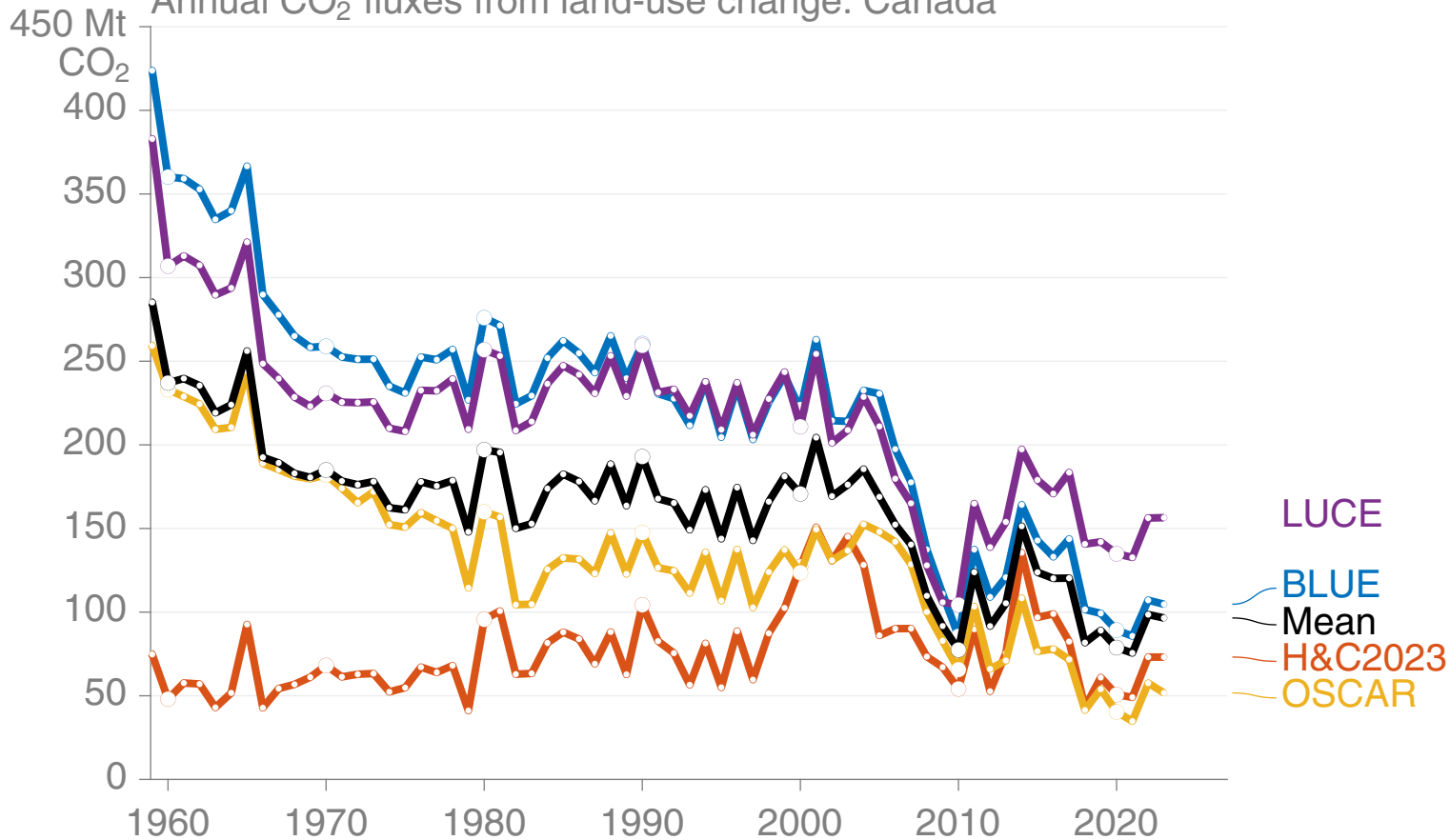
Annual CO 2 fluxes from land-use change: Canada
