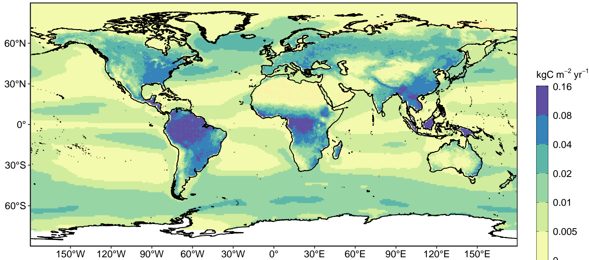
a CO 2 effect
