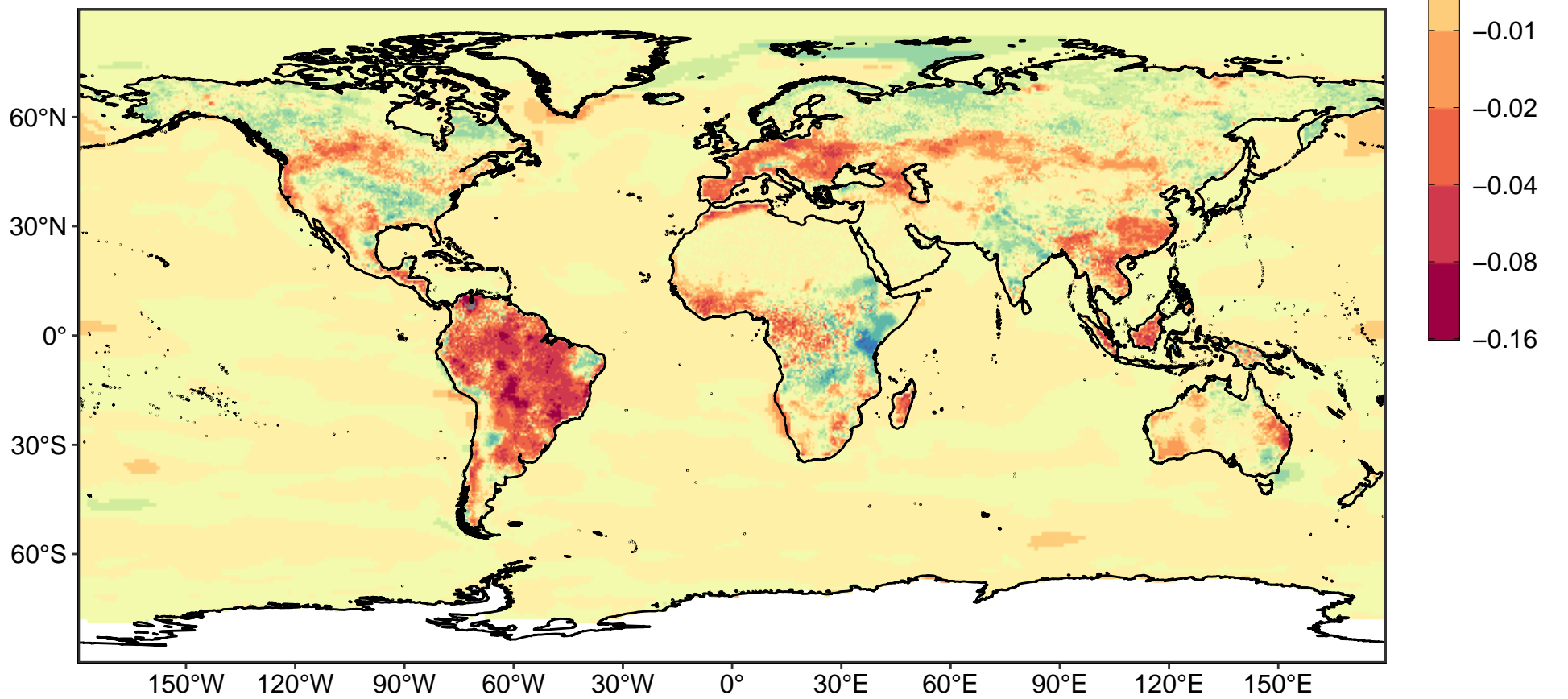
b Climate effect
