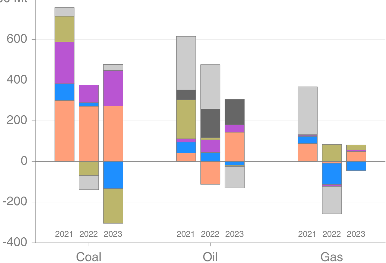
Changes in global fossil CO 2 emissions by region and fuel
