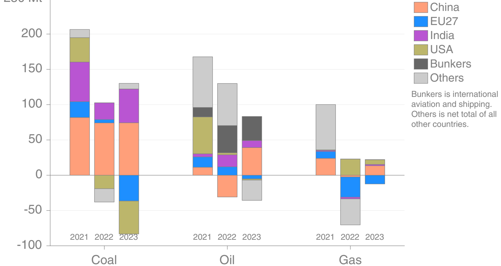
250 Mt Changes in global fossil CO 2 emissions by region and fuel
